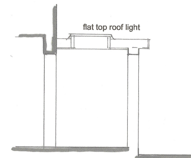
Sitting Room Link B-B
