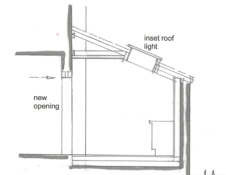
Section Through Kitchen A-A
