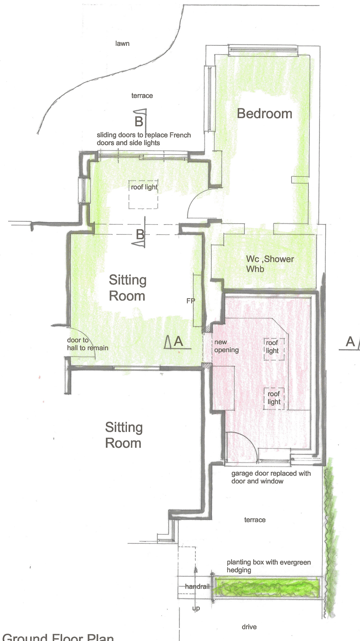
Ground Floor Plan of Annex
