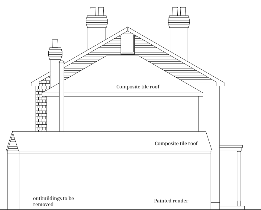
Existing South East Elevation 1:100
