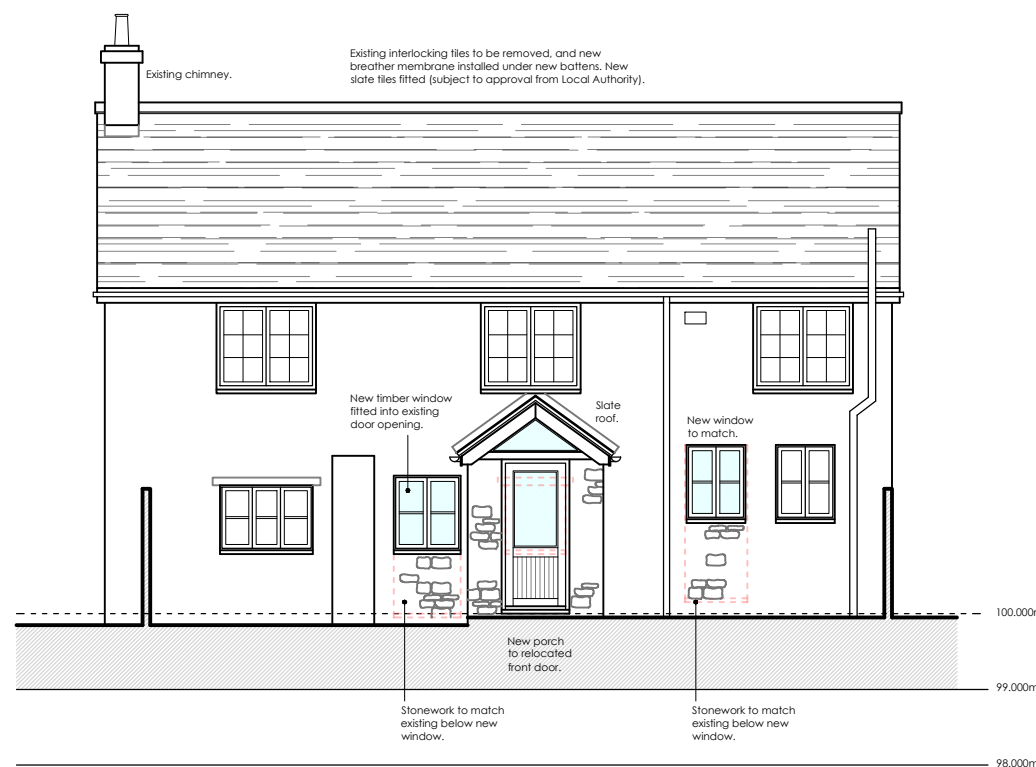
Proposed North-East Elevation 1:100
