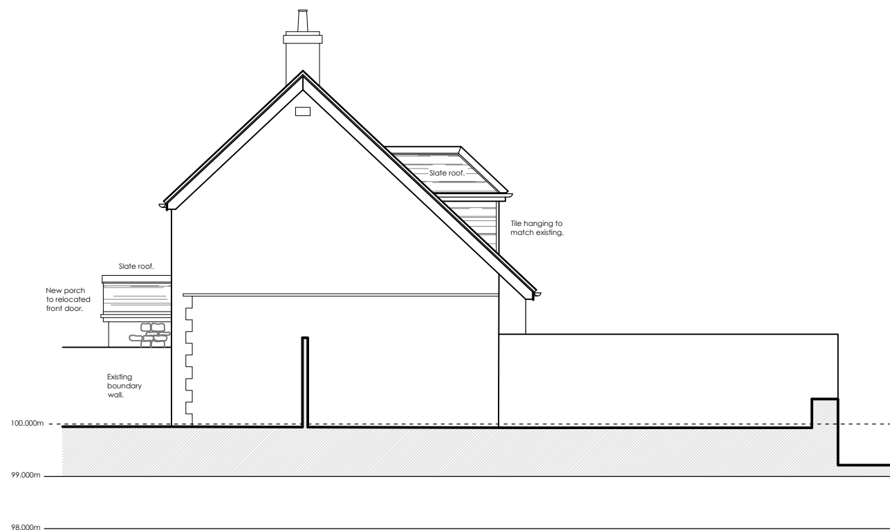
Proposed North-West Elevation 1:100
