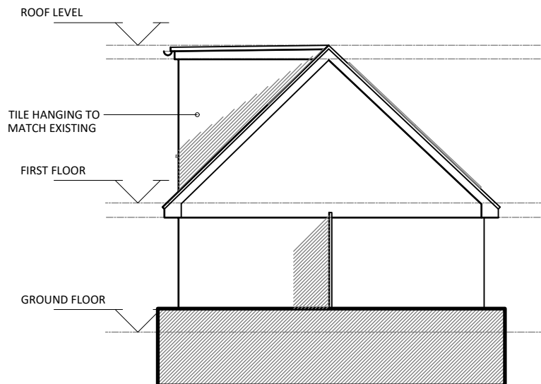
PROPOSED WEST ELEVATION 1:100 @ A4
