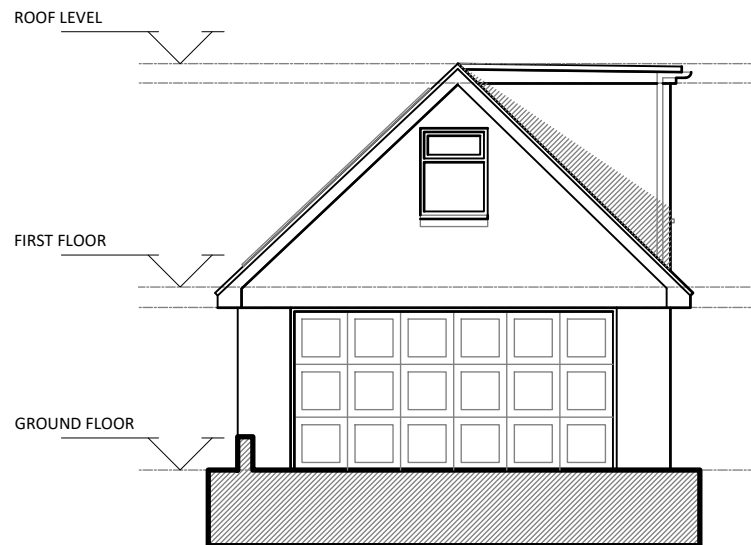
PROPOSED EAST ELEVATION 1:100 @ A4
