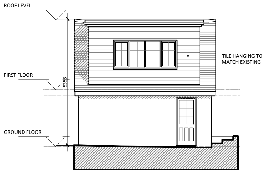
PROPOSED NORTH ELEVATION 1:100 @ A4
