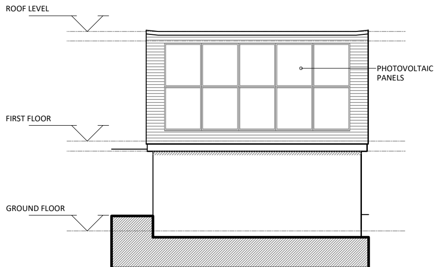
PROPOSED SOUTH ELEVATION 1:100 @ A4
