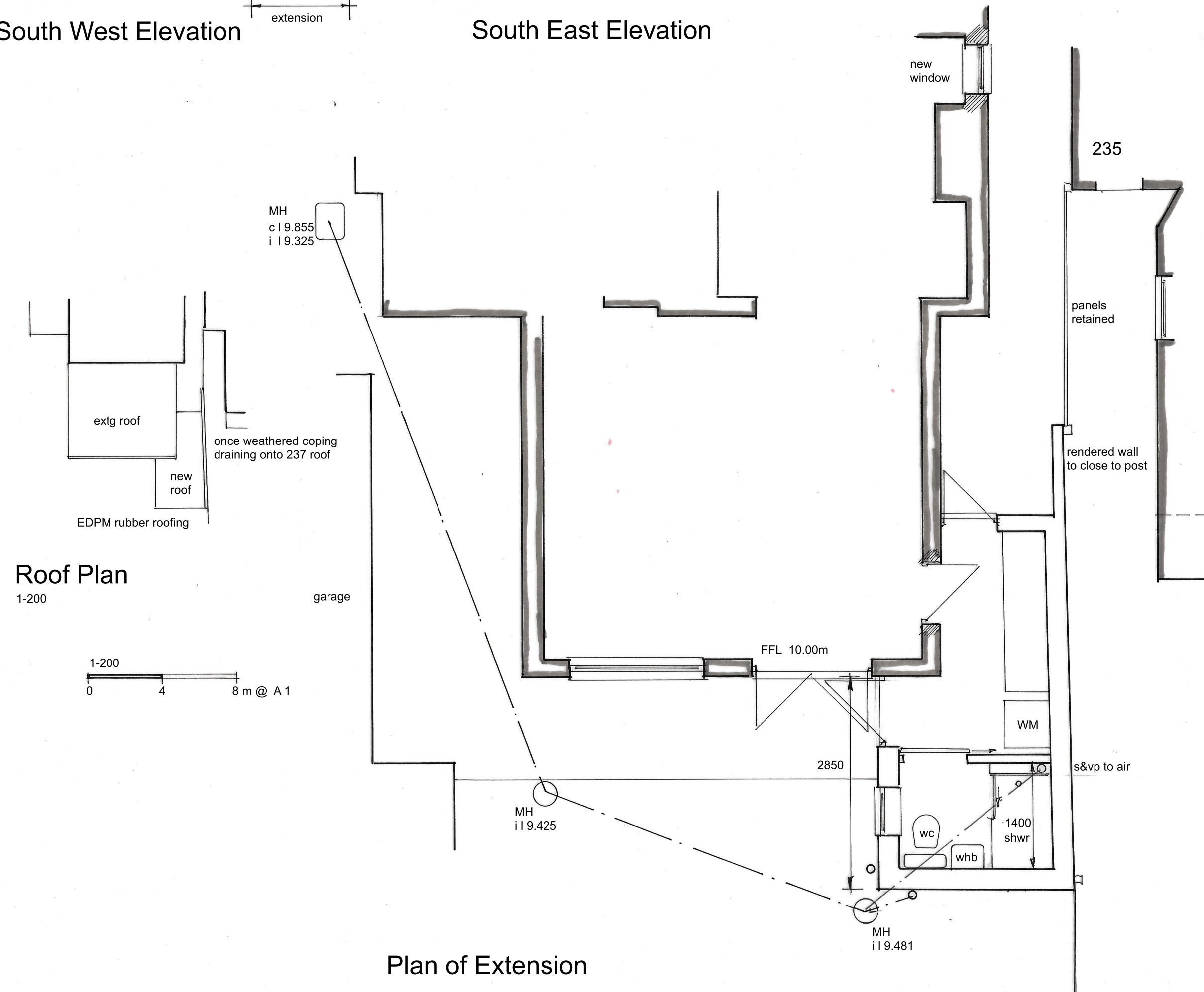
As Proposed
