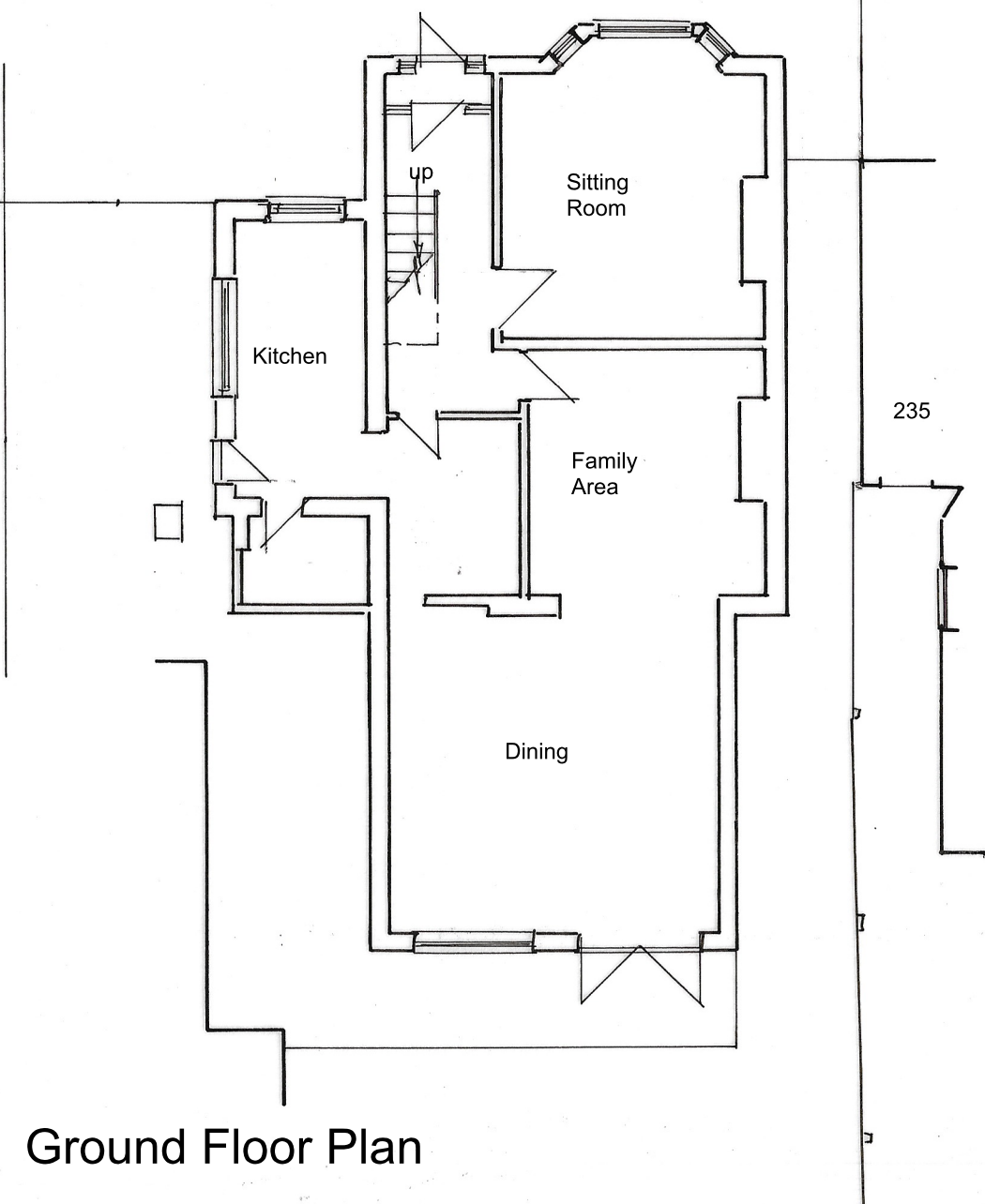
As Existing
