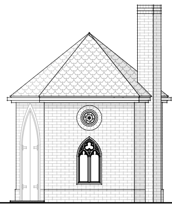
5 Proposed S-E Elevation Scale: 1:100
