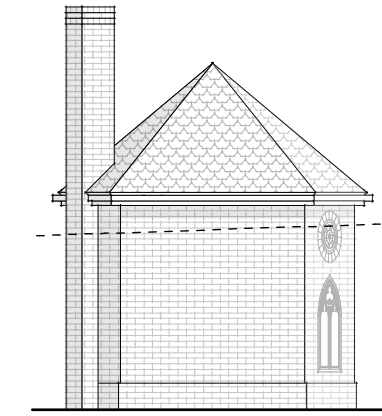
7 Proposed North Elevation Scale: 1:100
