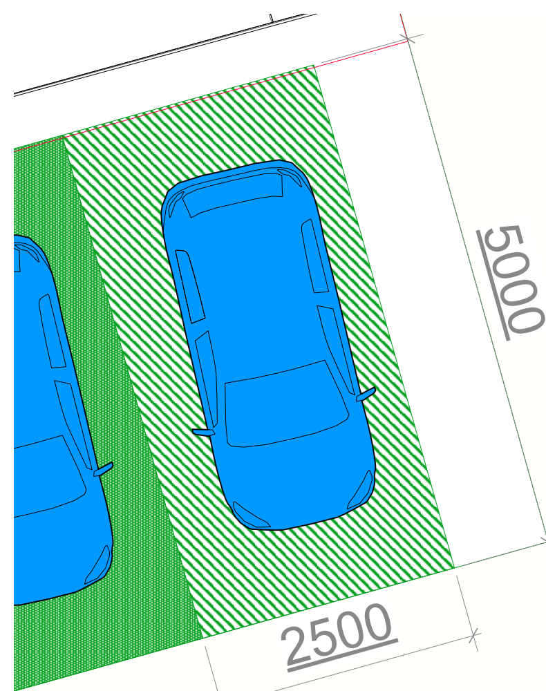
4 Pool Car Small x 4 Scale: 1:50
