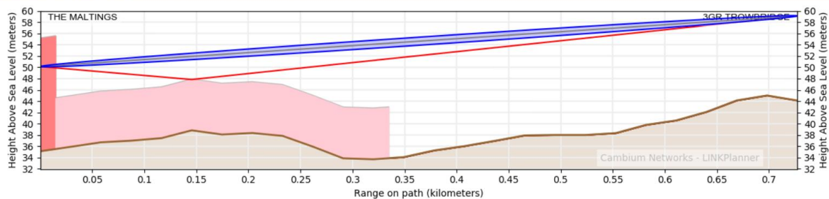
Profile: 0.727 kilometers, Non Line-of-Sight
