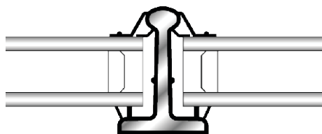
Heritage LC7 DG type lead covered steel glazing bar - double glazed
