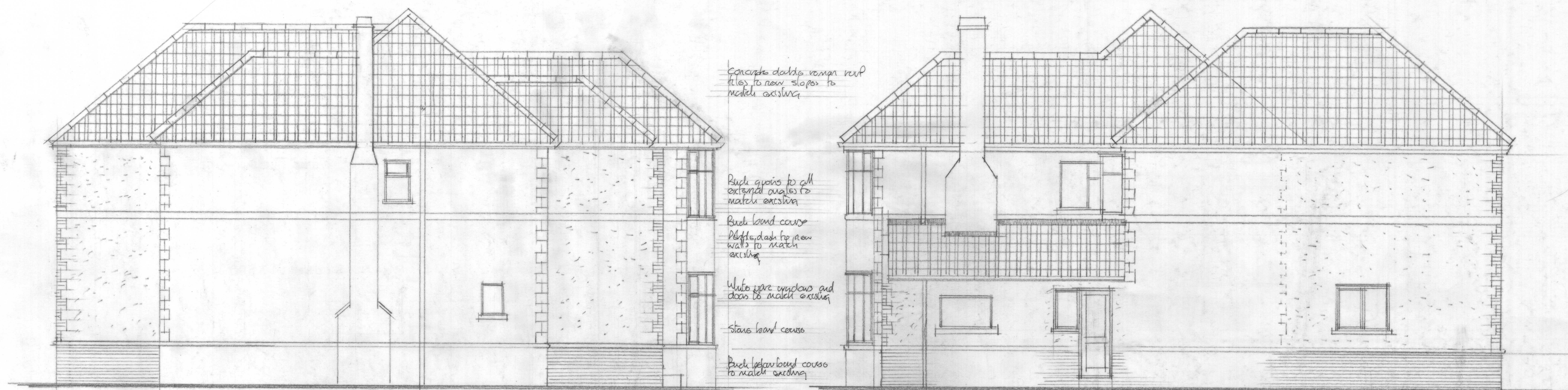
SOUTH ELEVATION
