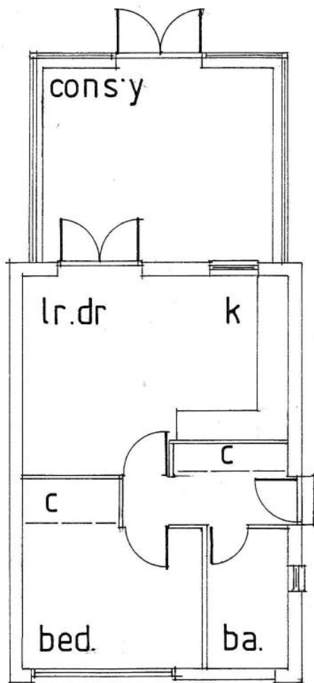
floor plan
