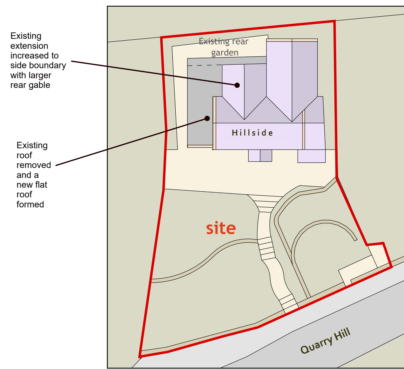
Proposed Layout 1 : 2 0 0
