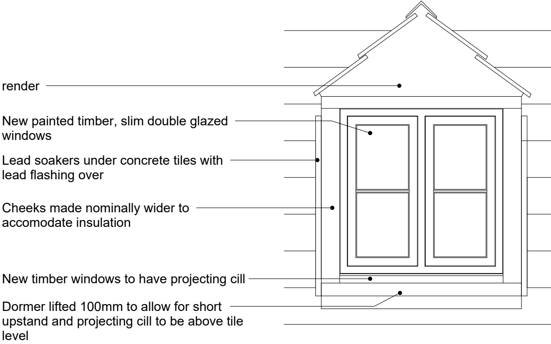
3 Proposed east dormer - front elevation 1 : 20
