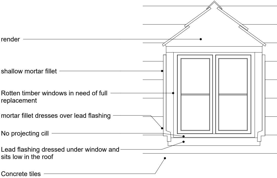
2 Existing east dormer - front elevation 1 : 20
