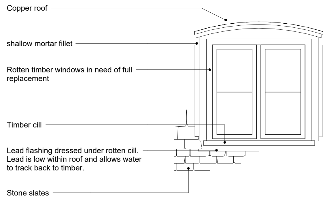
2 Existing west dormer - front elevation 1 : 20
