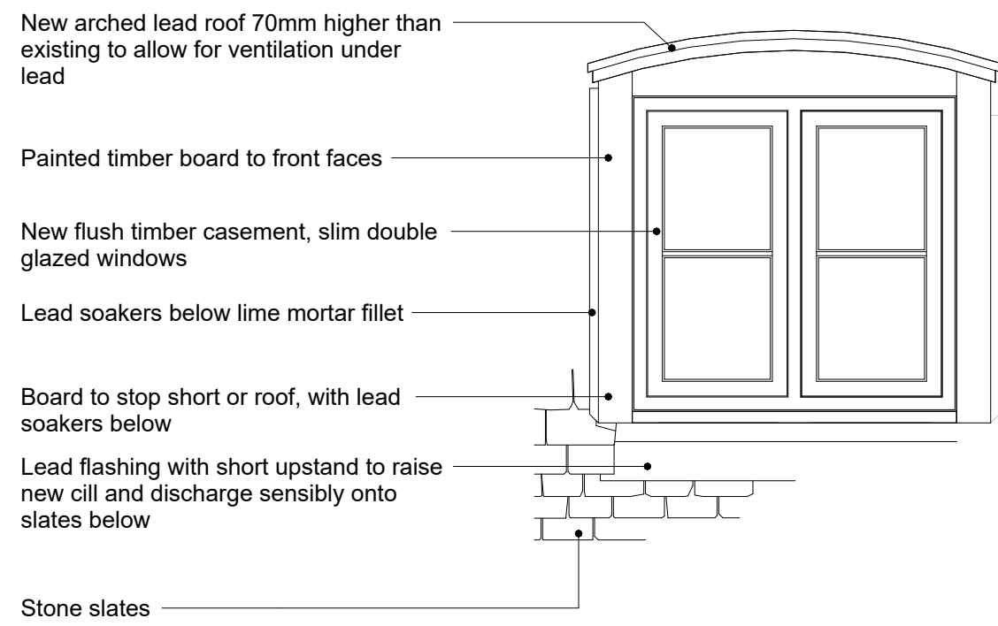
3 Proposed west dormer - front elevation 1 : 20
