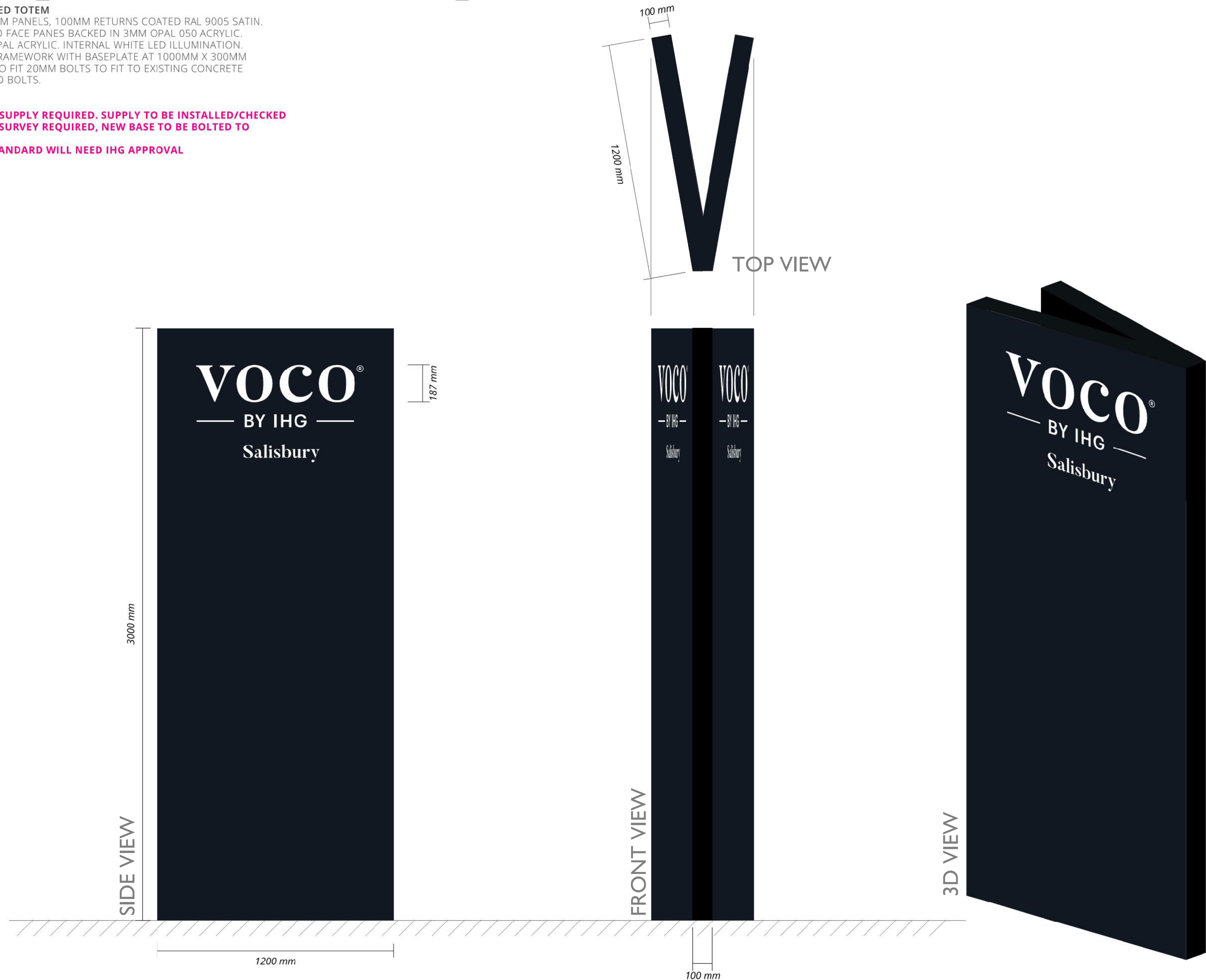
PROPOSED TOTEM SIGN @ 1:10 SCALE
