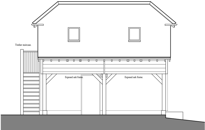
EXISTING NORTH-WEST ELEVATION (1:100 at A3)
