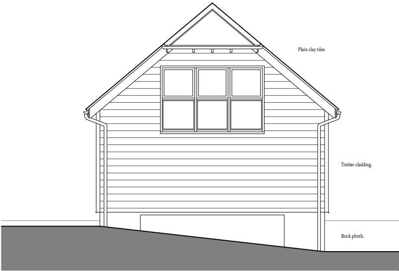
EXISTING SOUTH-WEST ELEVATION (1:100 at A3)
