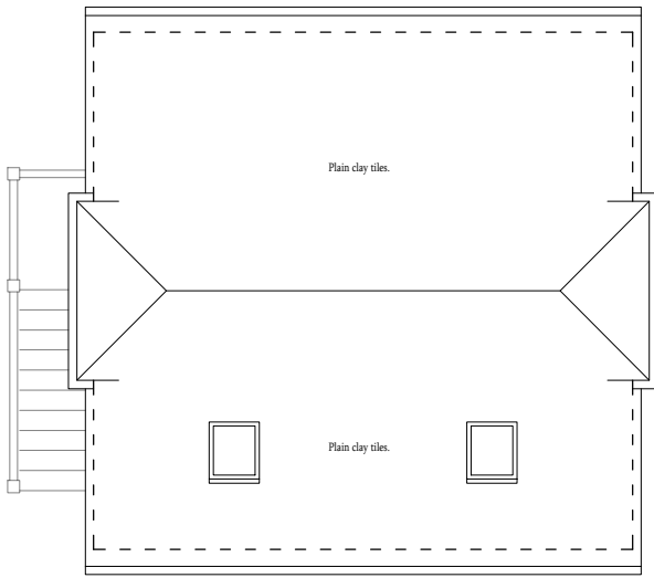
EXISTING ROOF PLAN (1:100 at A3)
