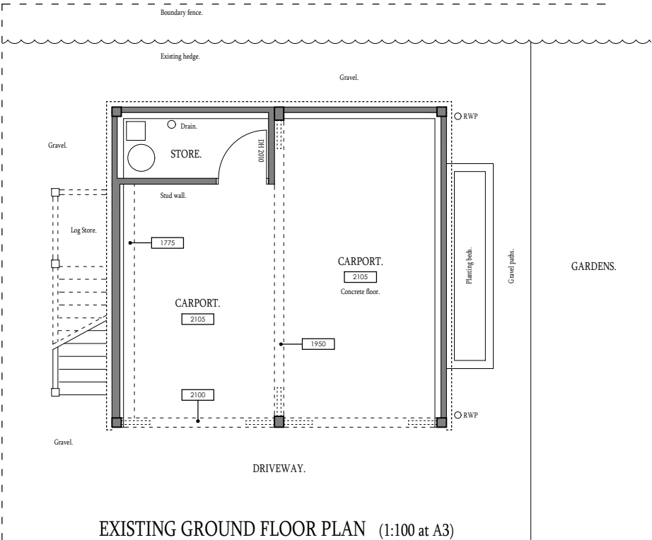
EXISTING GROUND FLOOR PLAN (1:100 at A3)
