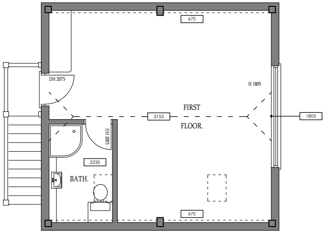
EXISTING FIRST FLOOR PLAN (1:100 at A3)
