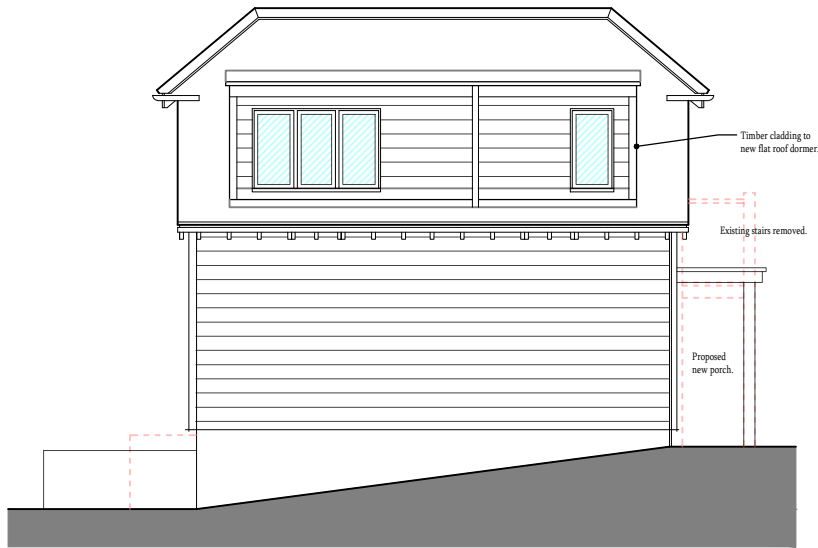
PROPOSED SOUTH-EAST ELEVATION (1:100 at A3)
