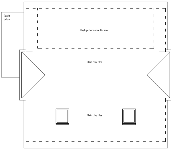
PROPOSED ROOF PLAN (1:100 at A3)
