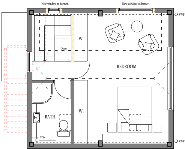
PROPOSED FIRST FLOOR PLAN (1:100 at A3)
