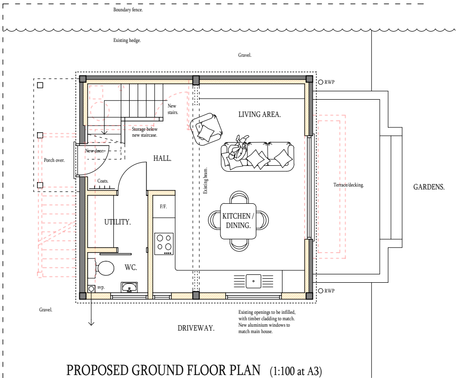
PROPOSED GROUND FLOOR PLAN (1:100 at A3)
