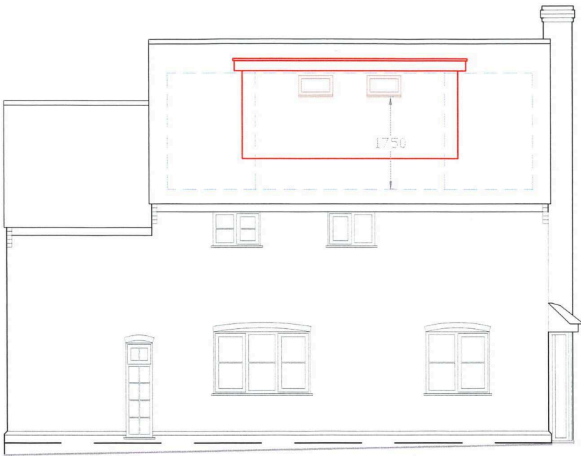
East Elevation
