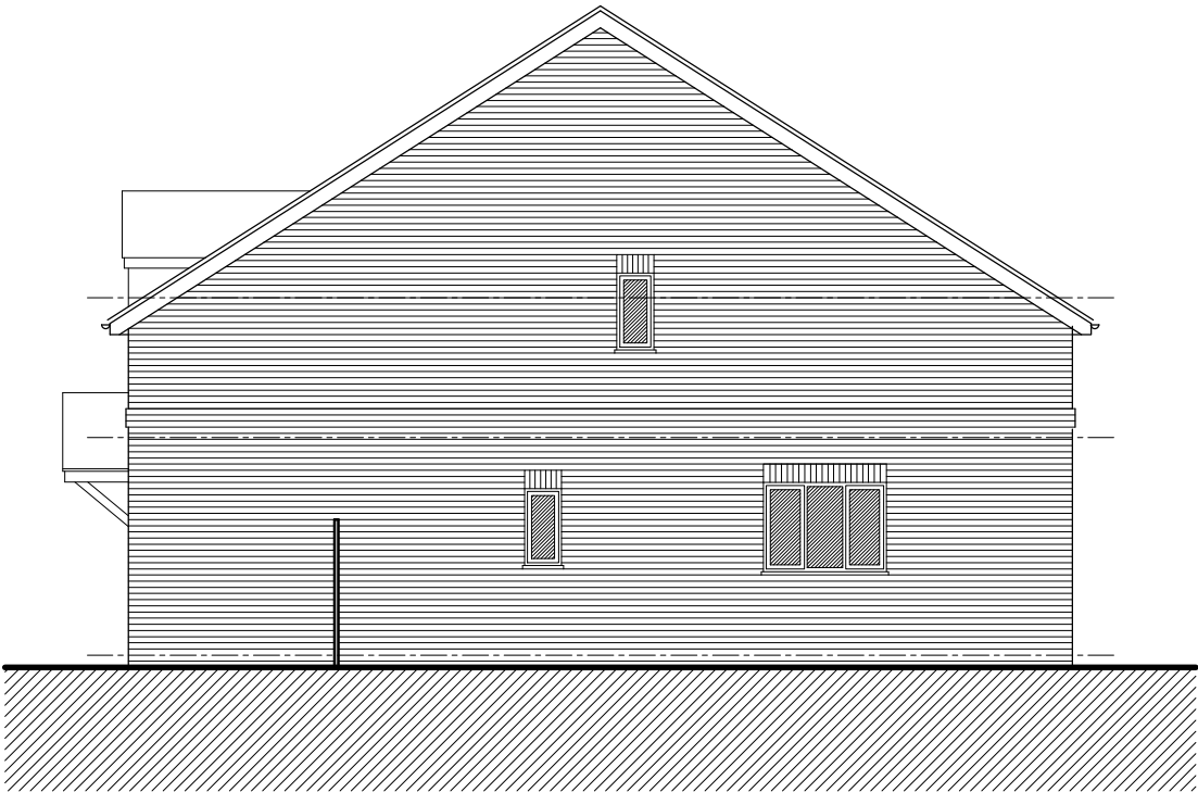
North Elevation
