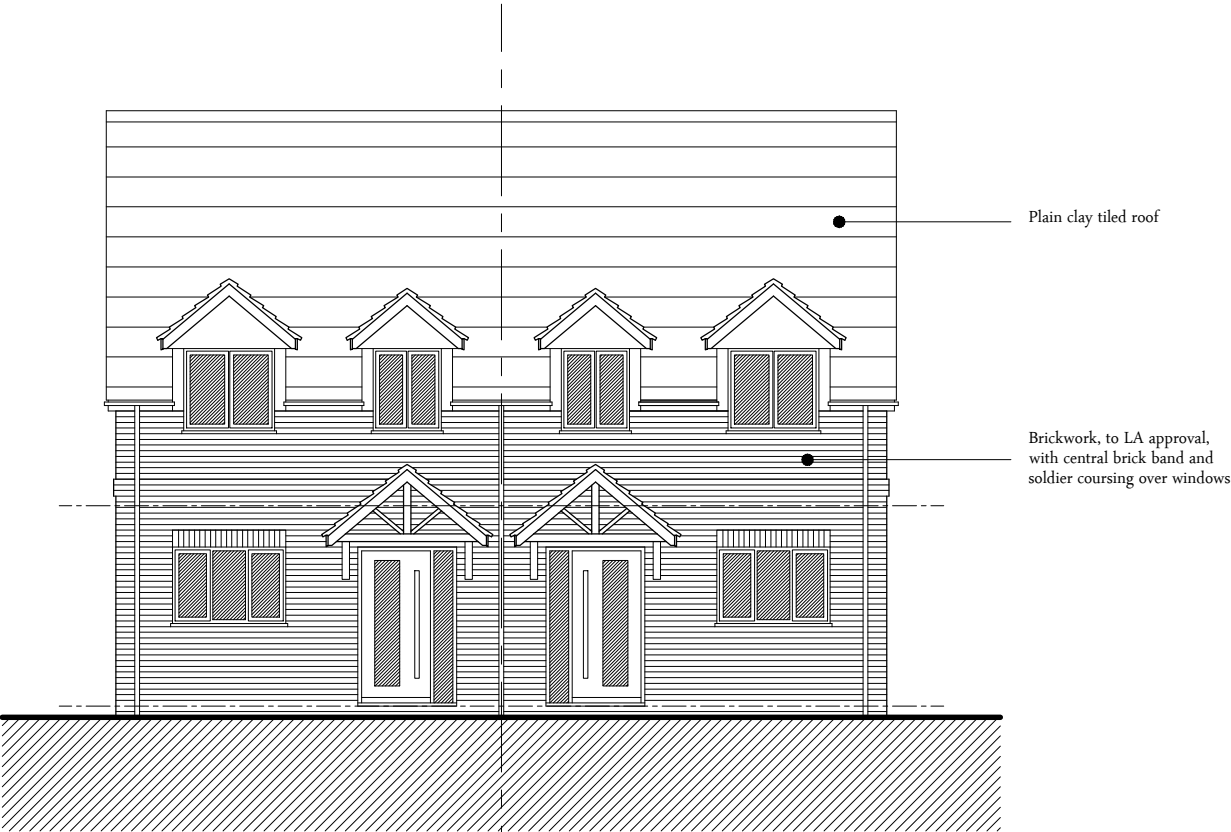
East Elevation
