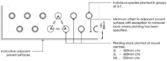
Detail 6 - Typical Shrub Planting Layout (N.T.S.)
