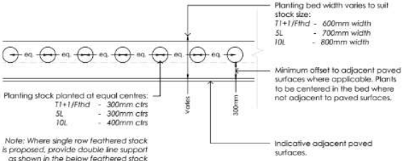
Detail 7 - Typical Single Row Hedgerow Layout (N.T.S.)
