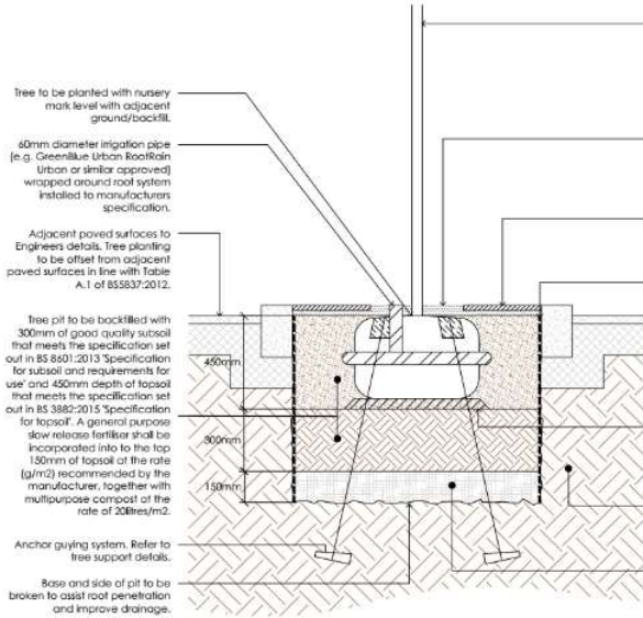
Detail 2 - Typical Tree Pit within Hard Landscape (N.T.S.)
