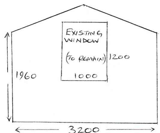
SOUTH ELEVATION
