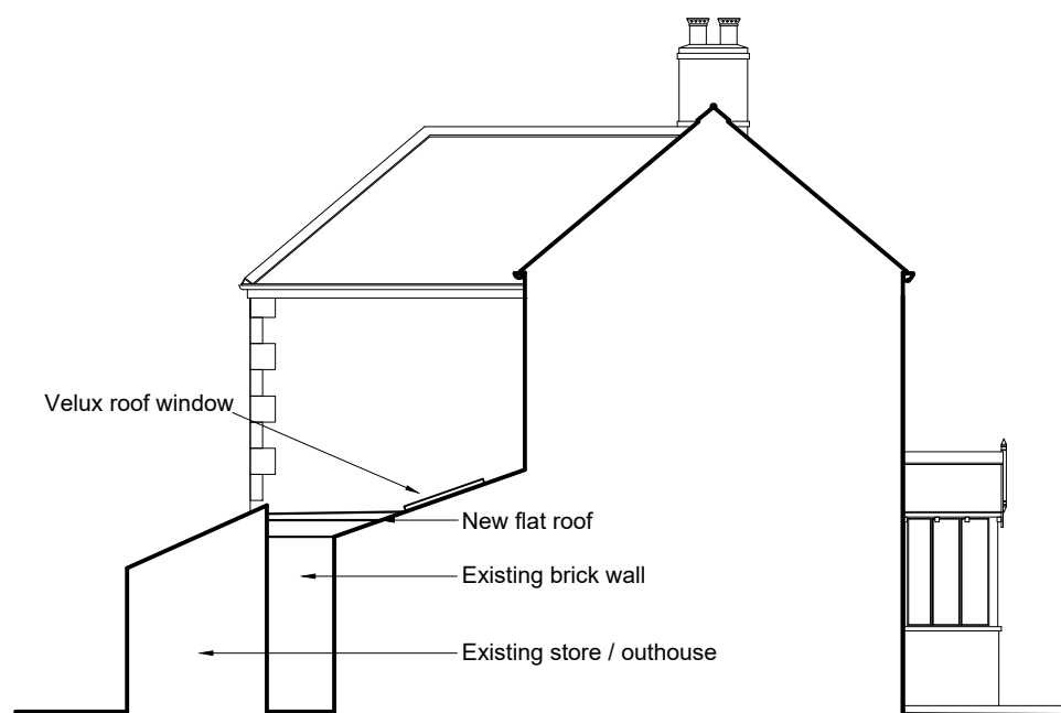
SOUTH WEST (Side)
