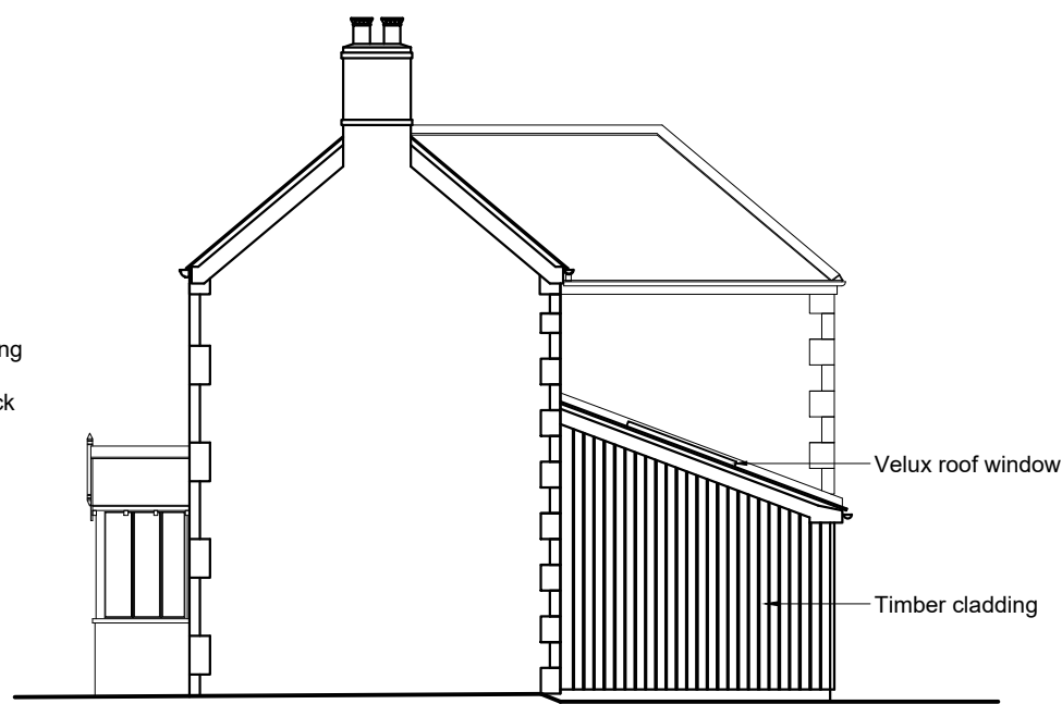
NORTH EAST (Side)
