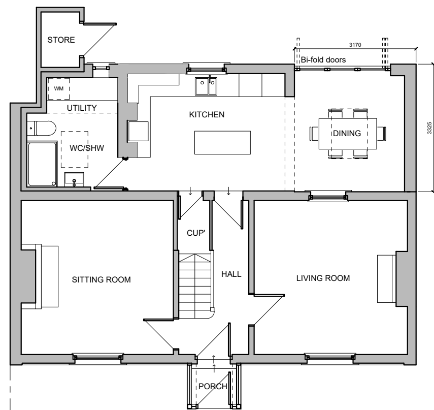
GROUND FLOOR PROPOSED FLOOR PLAN scale 1:100
