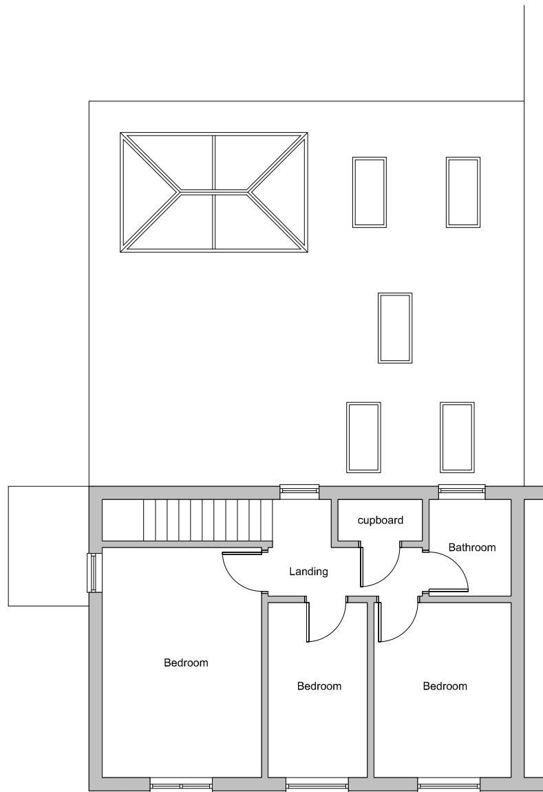
First Floor Plan as Planning Application PL/2025/02916 approved 14th May 2025
