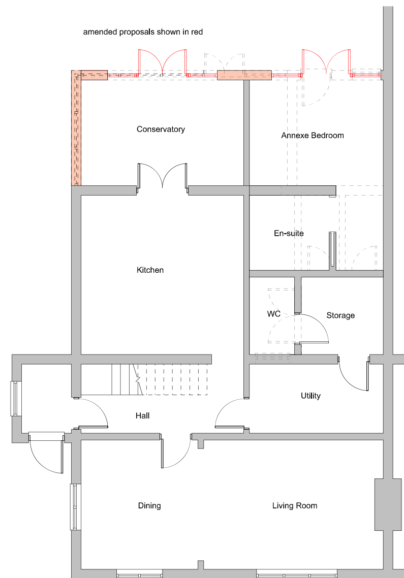
Ground Floor Plan - Proposed as Section 73 application June 2026
