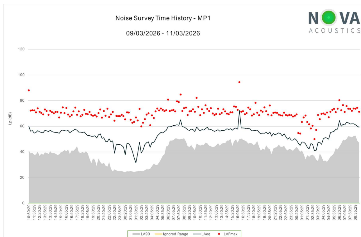
Figure 5 – MP1 Noise Survey Time History
