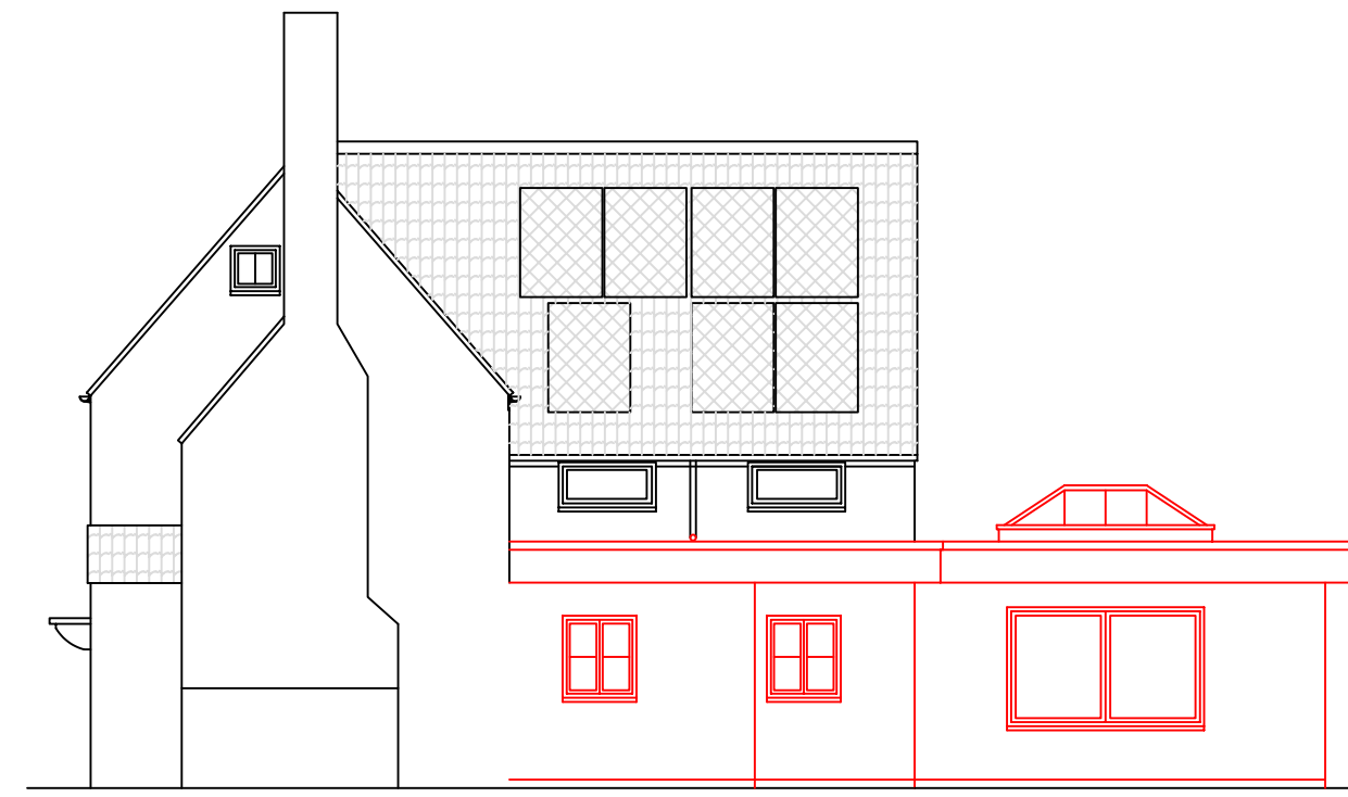
Proposed Side (East) Elevation 1:100
