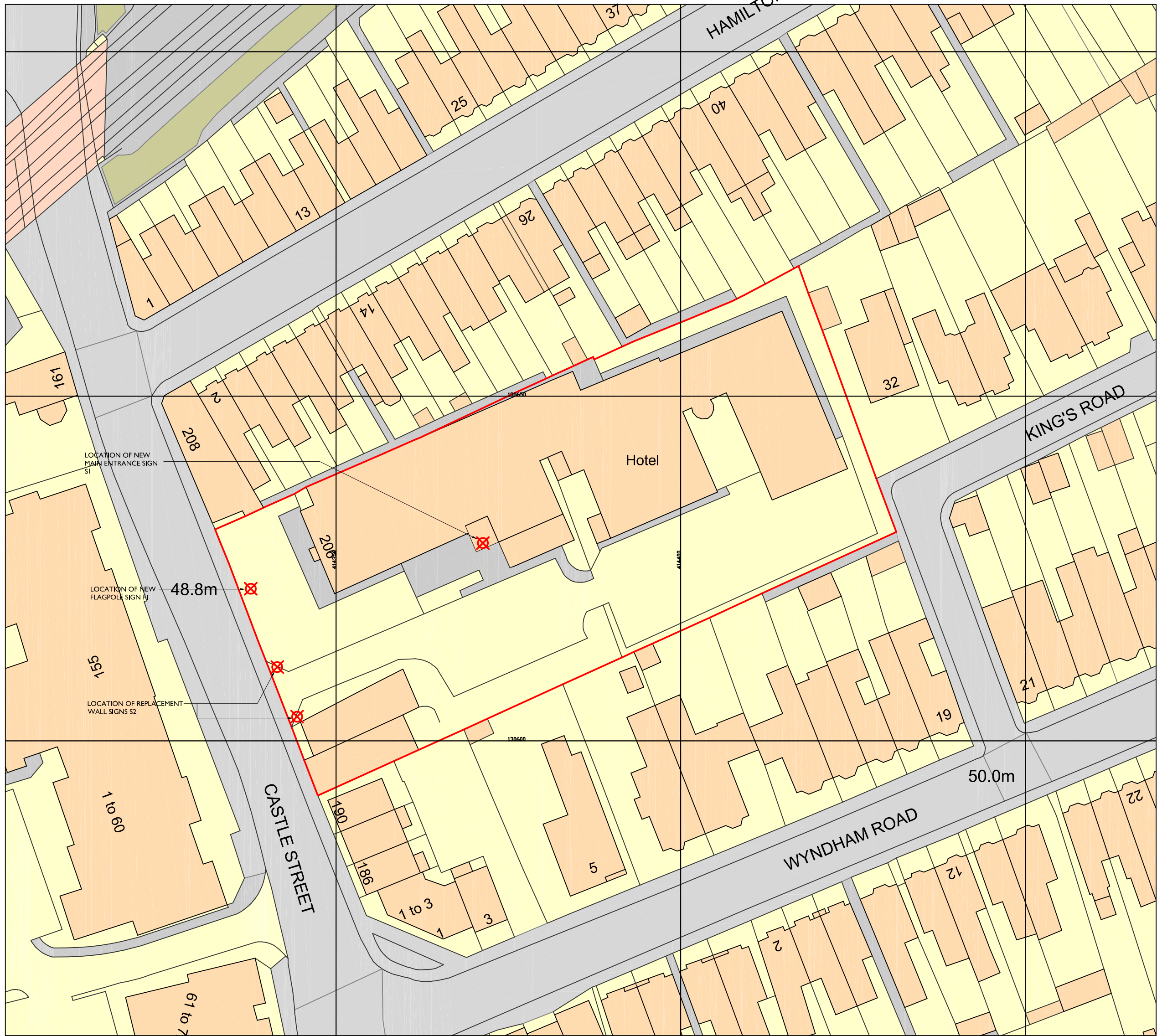
BLOCK PLAN 1:500 SCALE
