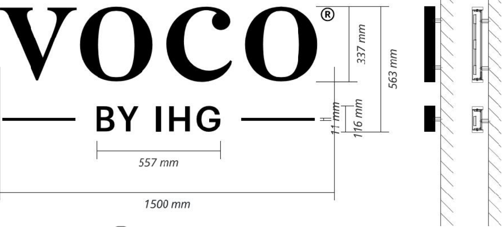
SIGN S1 @ 1:10 SCALE
