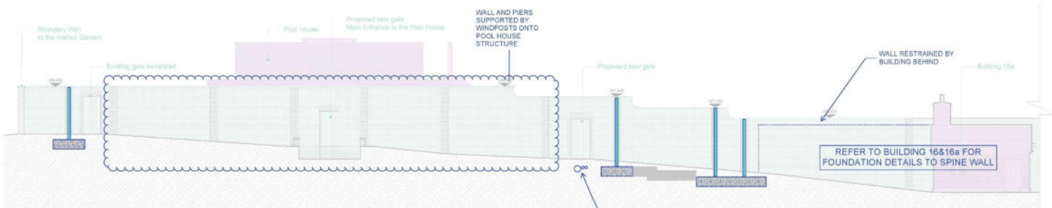
2 Proposed Spine Wall - First half of Elevation to North Scale 1:100 @ A1, 1:200 @ A3
