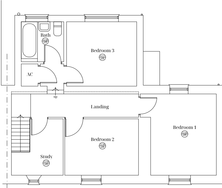
Proposed First Floor Plan (unchanged) 1:100
