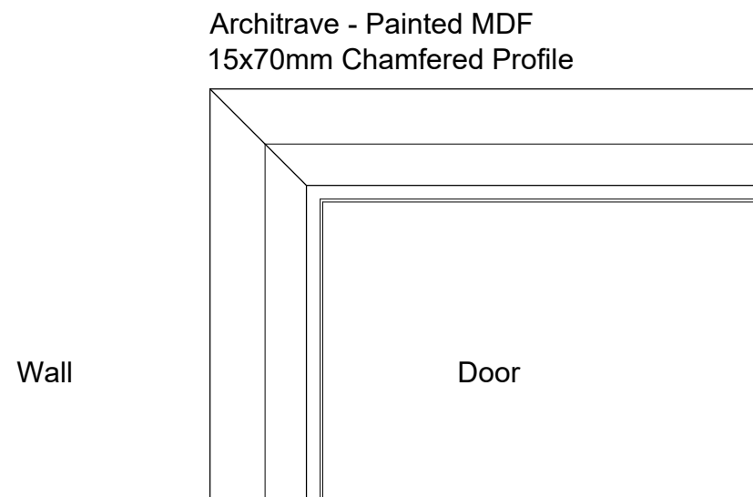
INTERNAL JOINARY - ARCHITRAVE Scale 1:5
