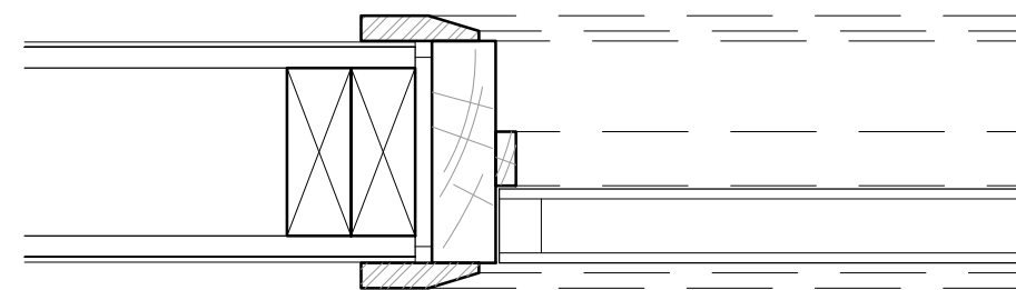
INTERNAL JOINARY - DOOR JAMB Scale 1:5
