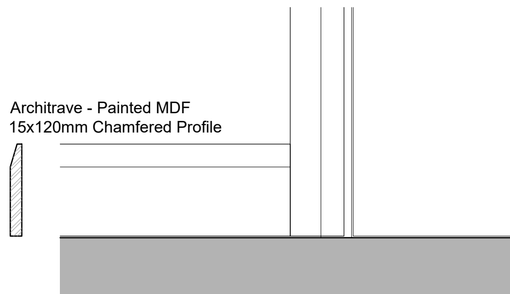
INTERNAL JOINARY - SKIRTING Scale 1:5
