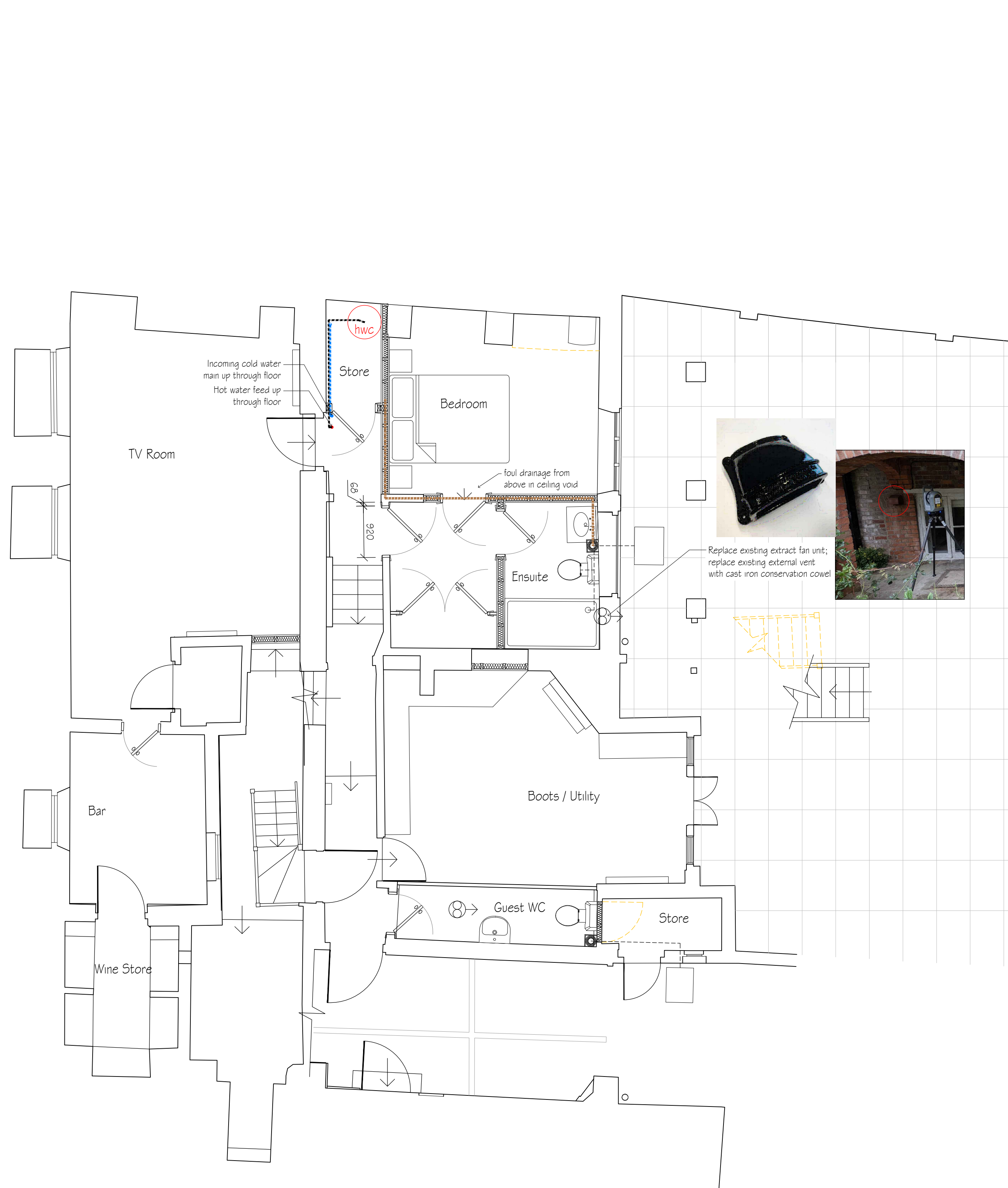
LOWER GROUND FLOOR 1:50
