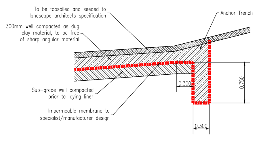
TYPICAL IMPERMEABLE MEMBRANE TO PERMANENT WATER BODY DETAIL
