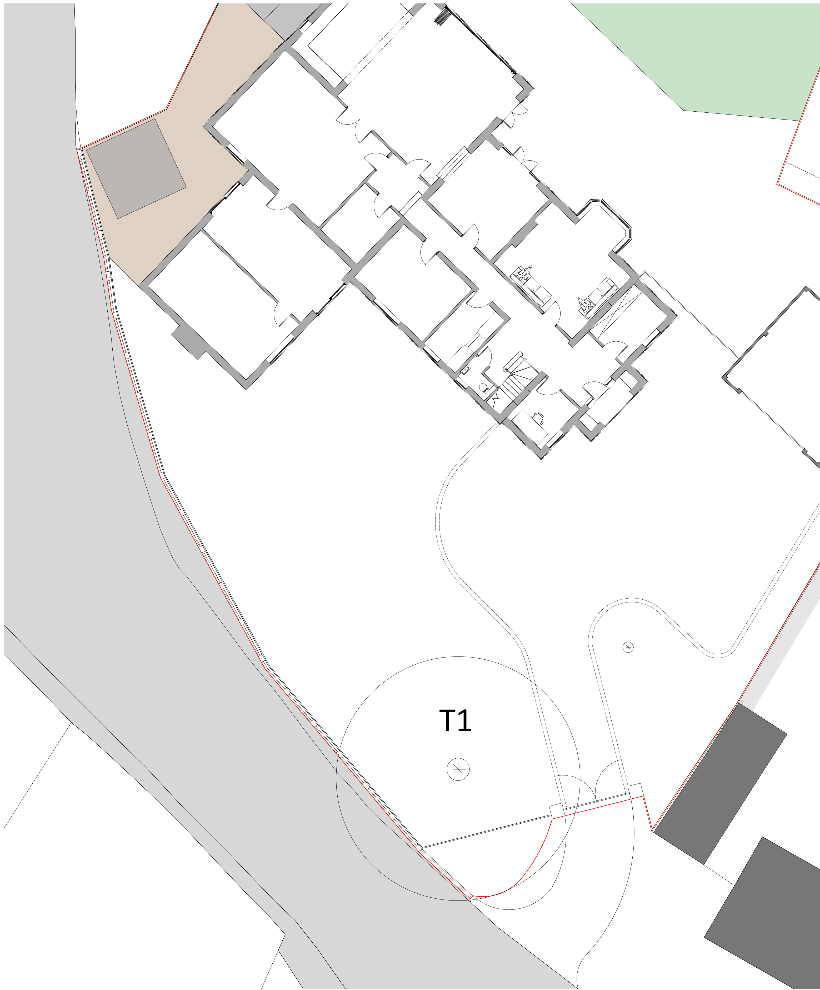
PLN 01 PROPOSED SITE PLAN 1:100
