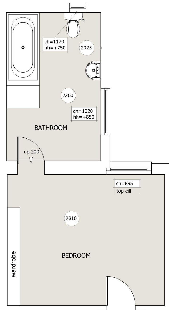
EXISTING LAYOUT
