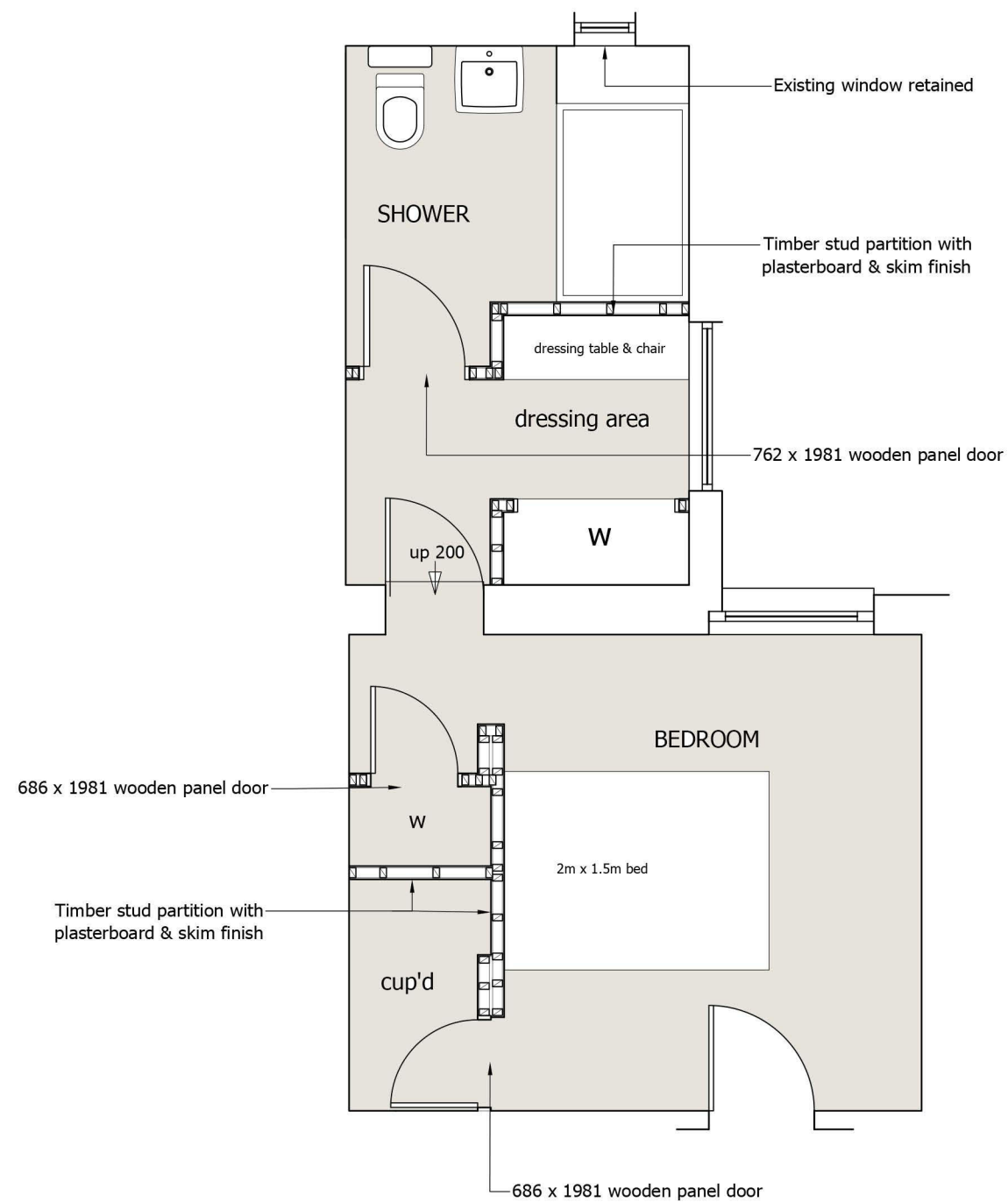
PROPOSED LAYOUT
