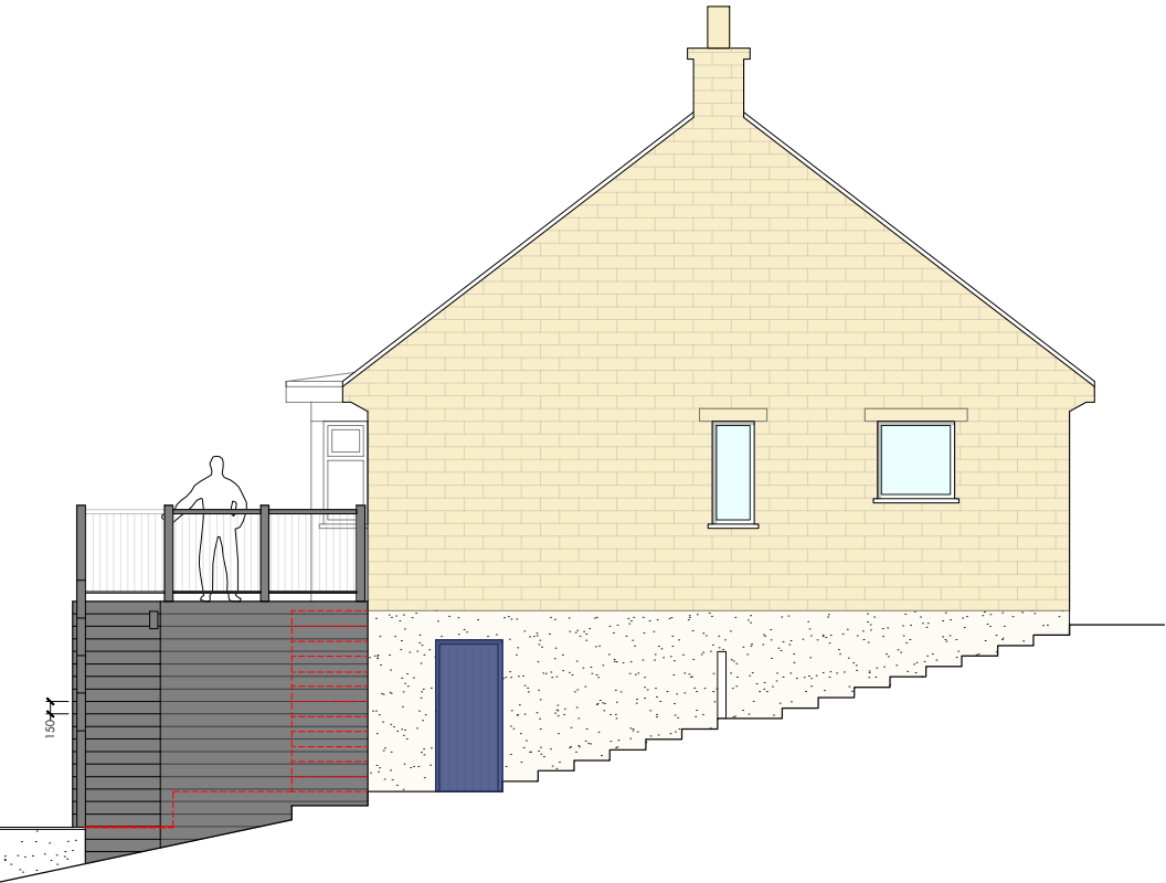
03 PROPOSED SIDE [NORTH-WEST] ELEVATION 1:100
