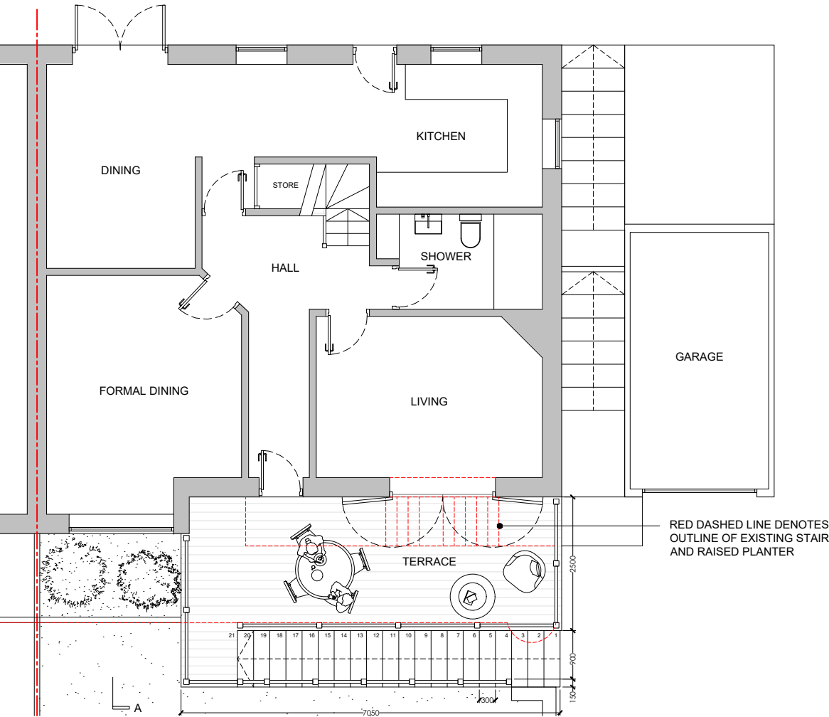
01 PROPOSED GROUND FLOOR PLAN 1:100
