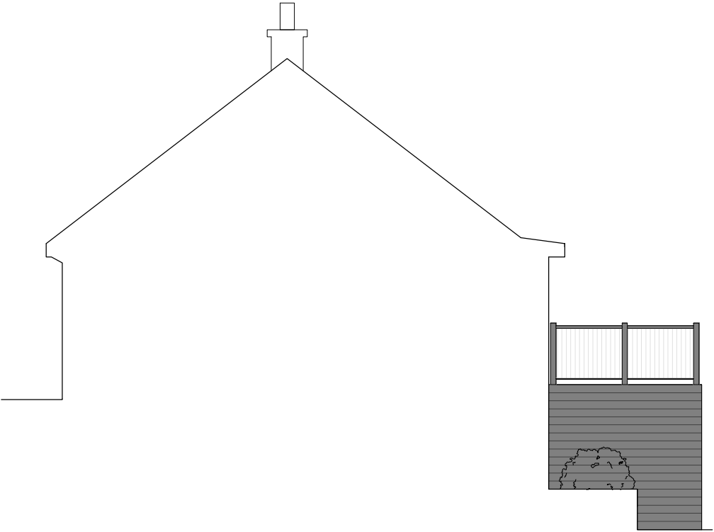
04 PROPOSED SIDE [SOUTH-EST] SECTION AA 1:100
