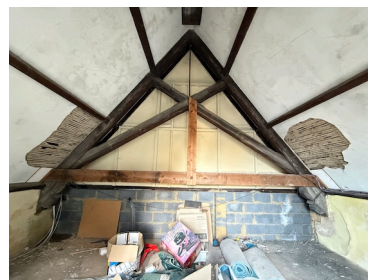
Fig 18 – Roof Void / Toilet Block: Truss Detail
