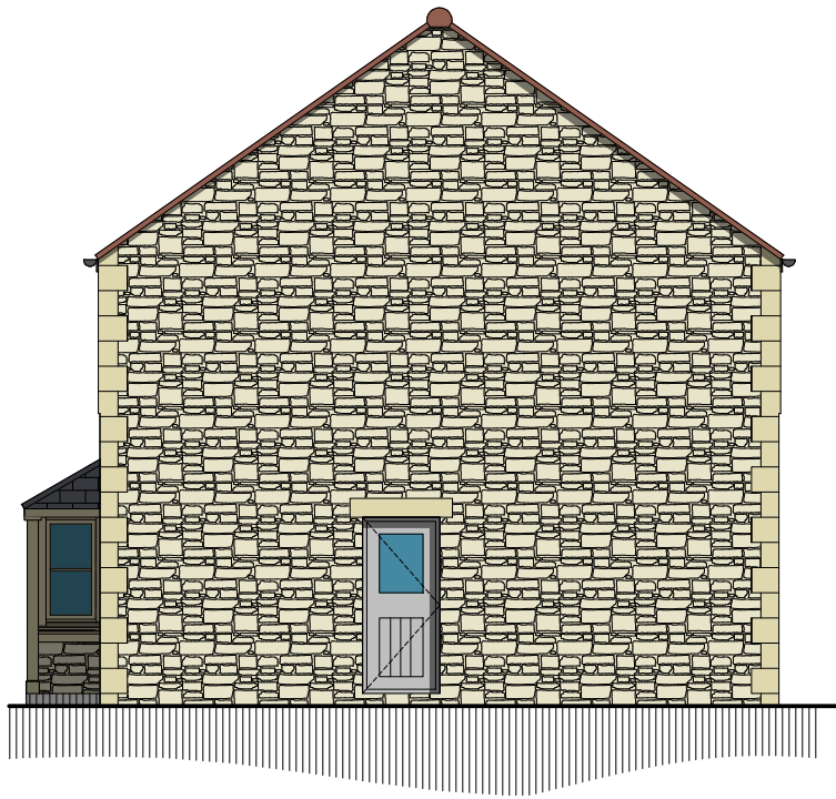
Side Elevation - Plots 6, 8 & 9 Proposed
