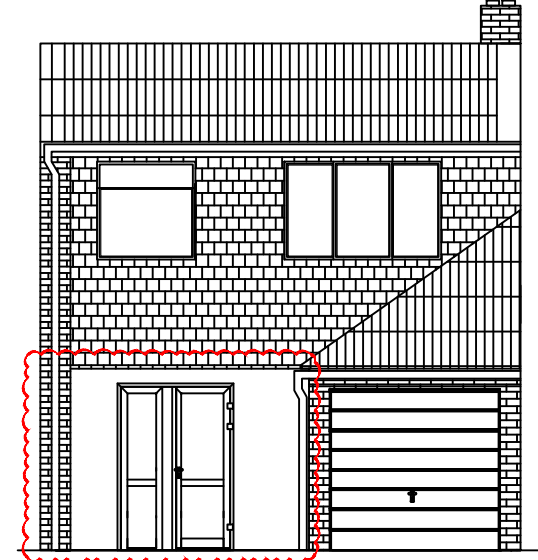
08 EXISTING WEST ELEVATION - 1 : 50 @ A3
