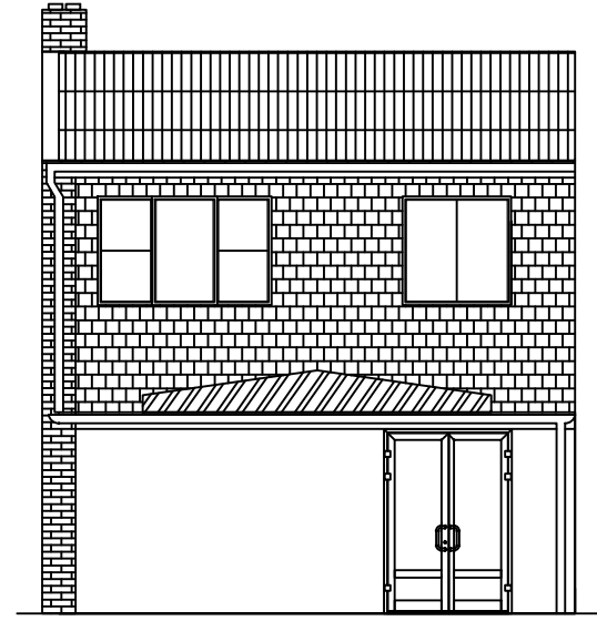
06 EXISTING EAST ELEVATION - 1 : 50 @ A3 No development on rear side
