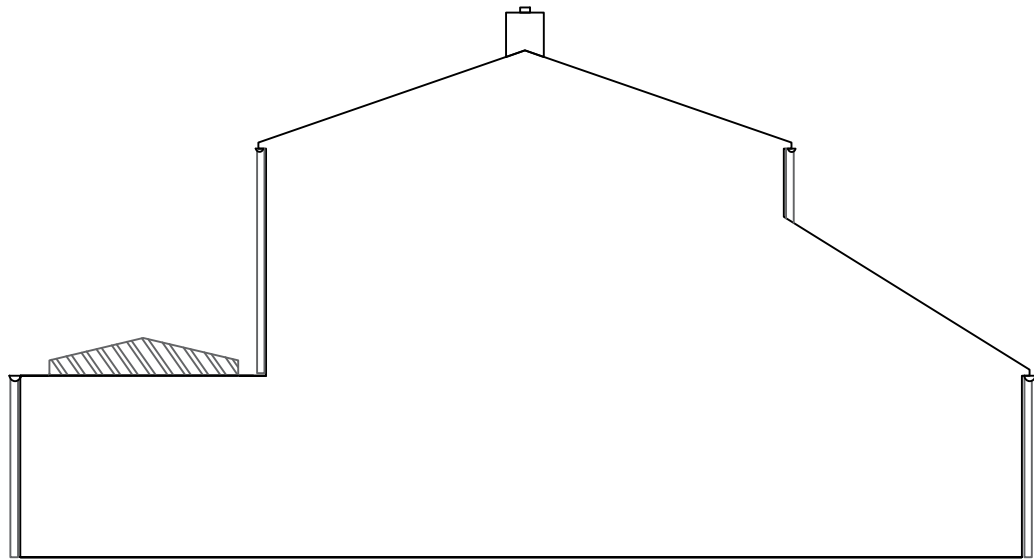
07 EXISTING NORTH ELEVATION - 1 : 50 @ A3
