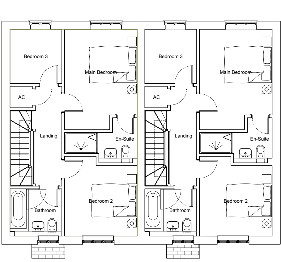
First Floor Plan - Plots 5 & 6 Proposed
