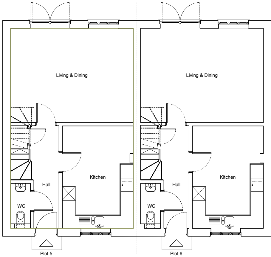
Ground Floor Plan - Plots 5 & 6 Proposed
