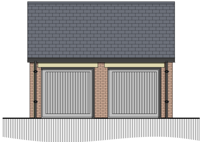
Front Elevation - Double Garage - Brick Finish Proposed
