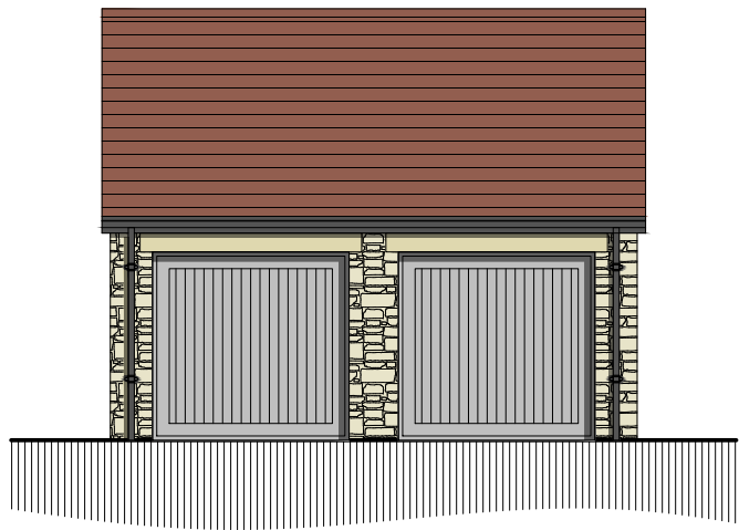
Front Elevation - Double Garage - Stone Finish Proposed
