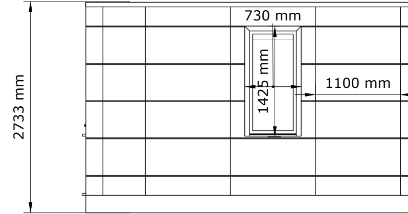
PROPOSED SIDE ELEVATION - Scale 1:50
