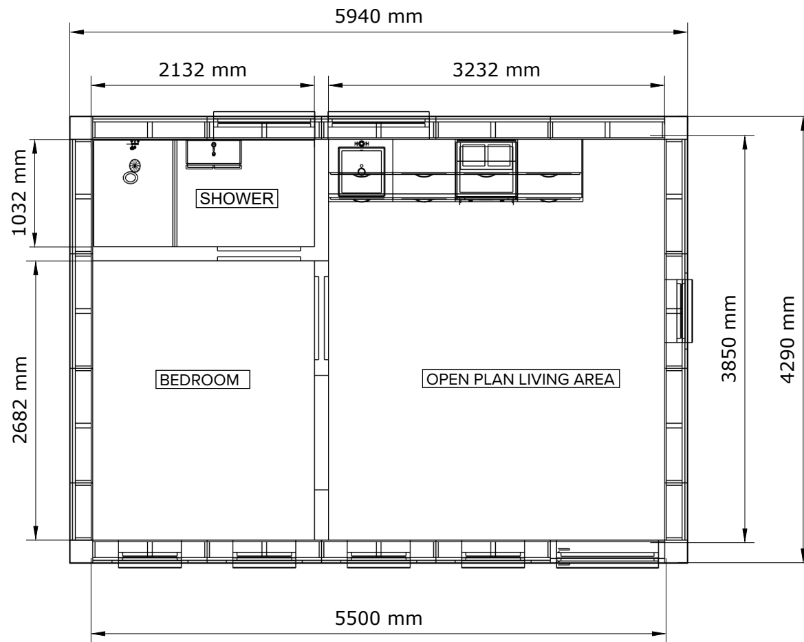
PROPOSED FLOOR PLAN - Scale 1:50
