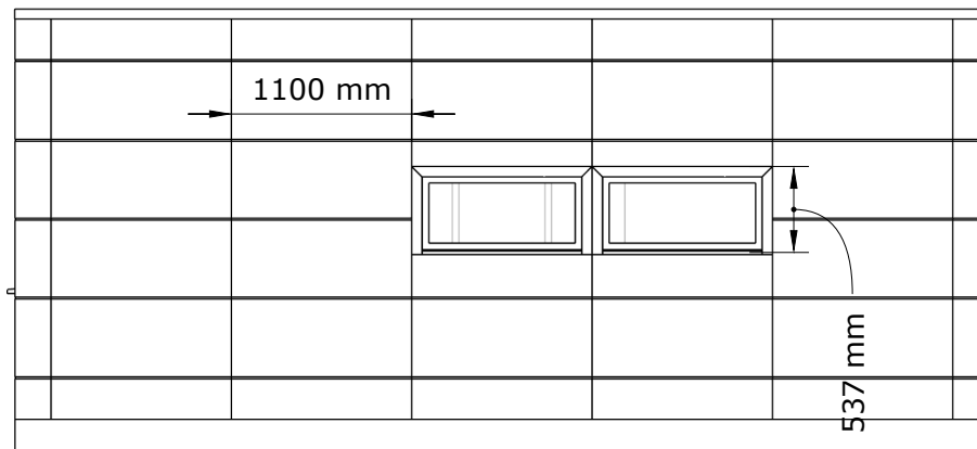
PROPOSED REAR ELEVATION - Scale 1:50
