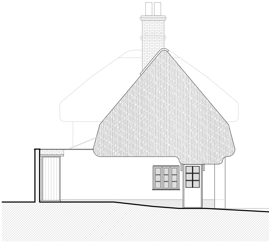
North Elevation
