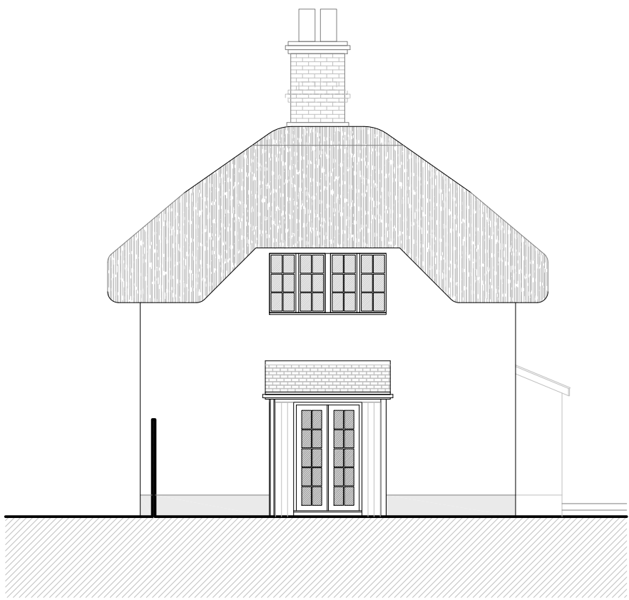
South Elevation
