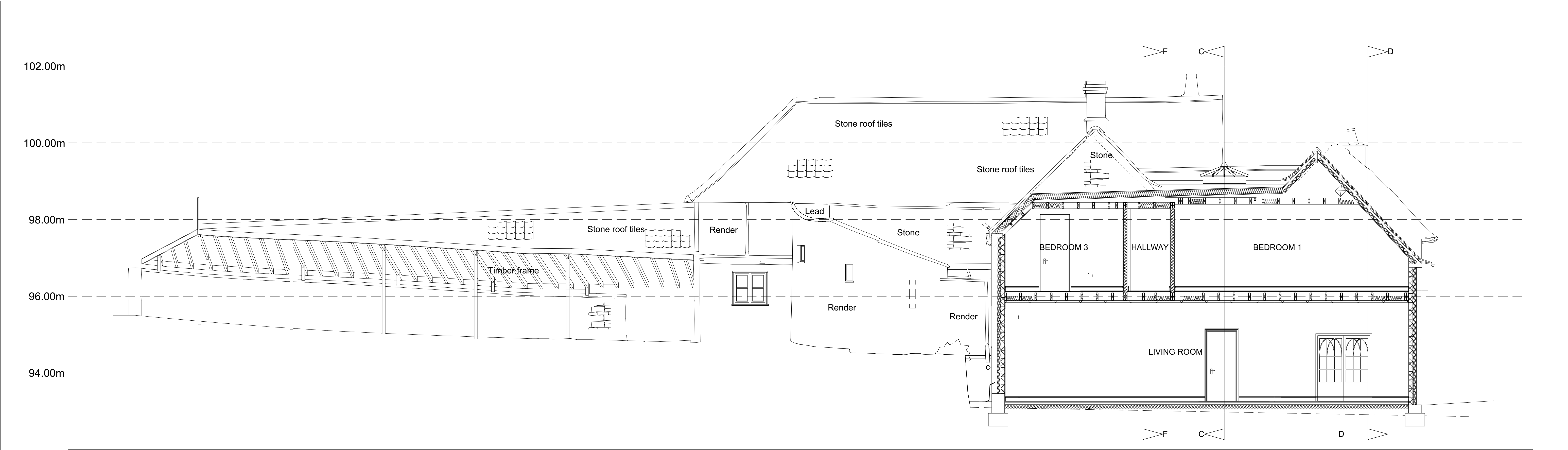
Section AA
