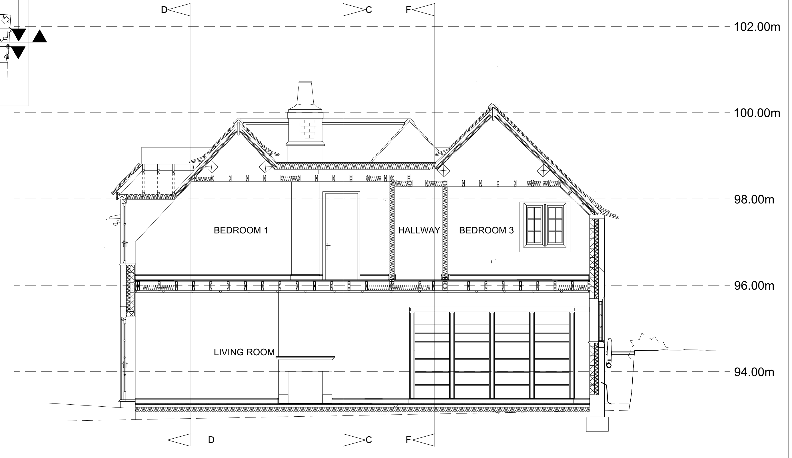
Section BB
