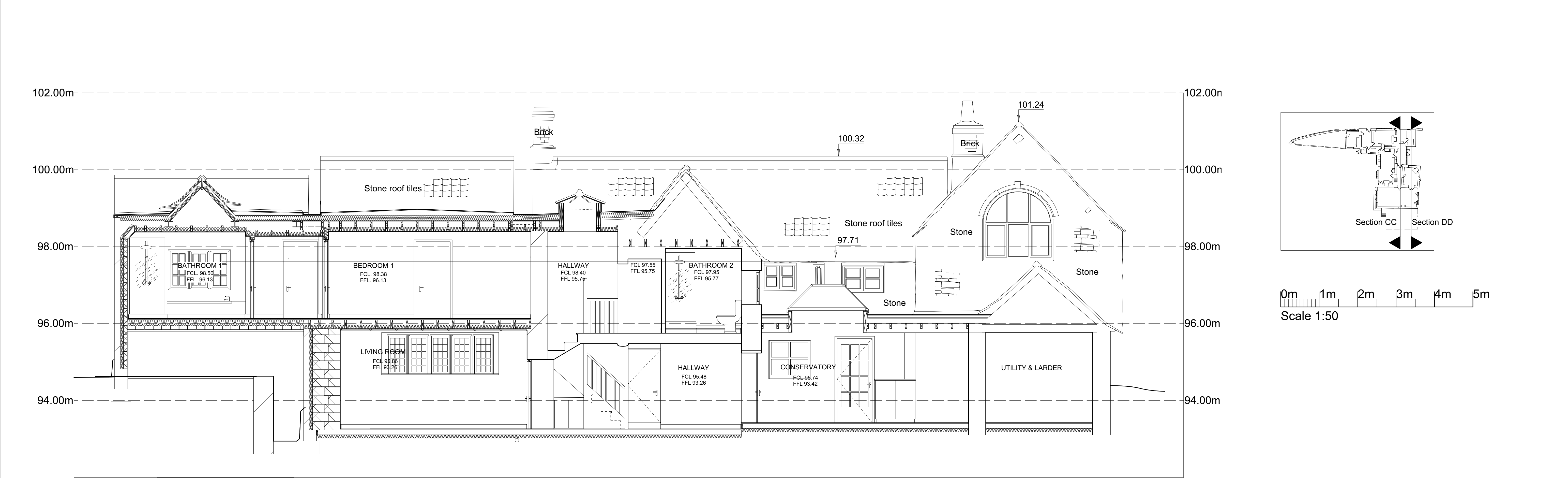
Datum line 92.00m House Section CC
