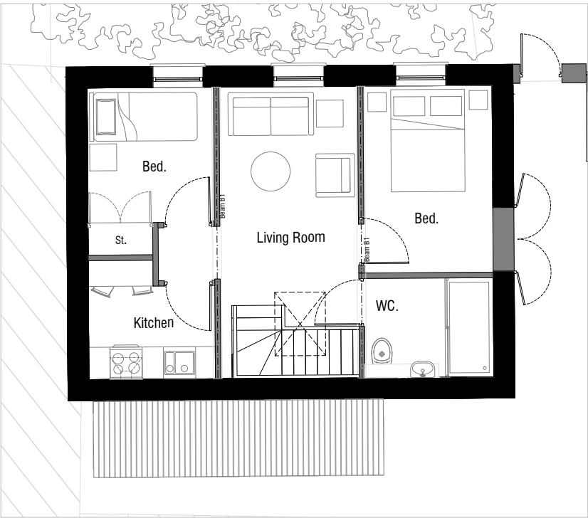
05 - First Floor Plan
