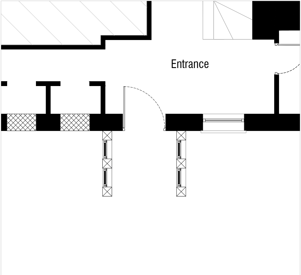
04 - Proposed Detail Plan (Cut through Windows)
