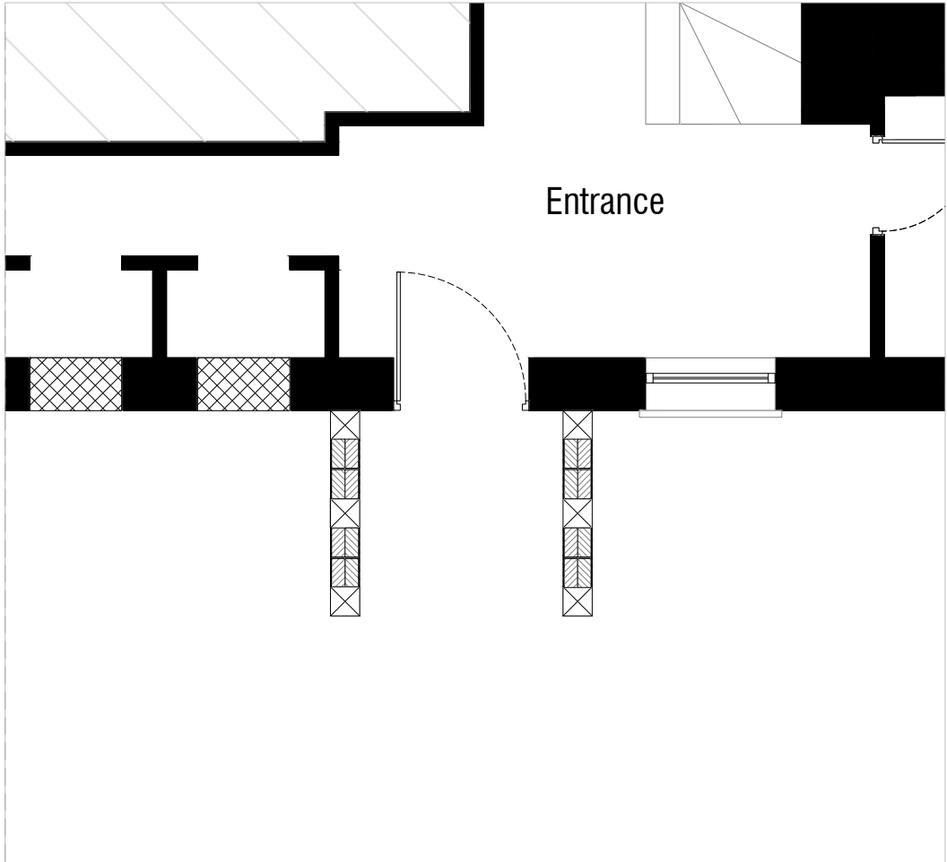
03 - Proposed Detail Plan (Cut through Wall)
