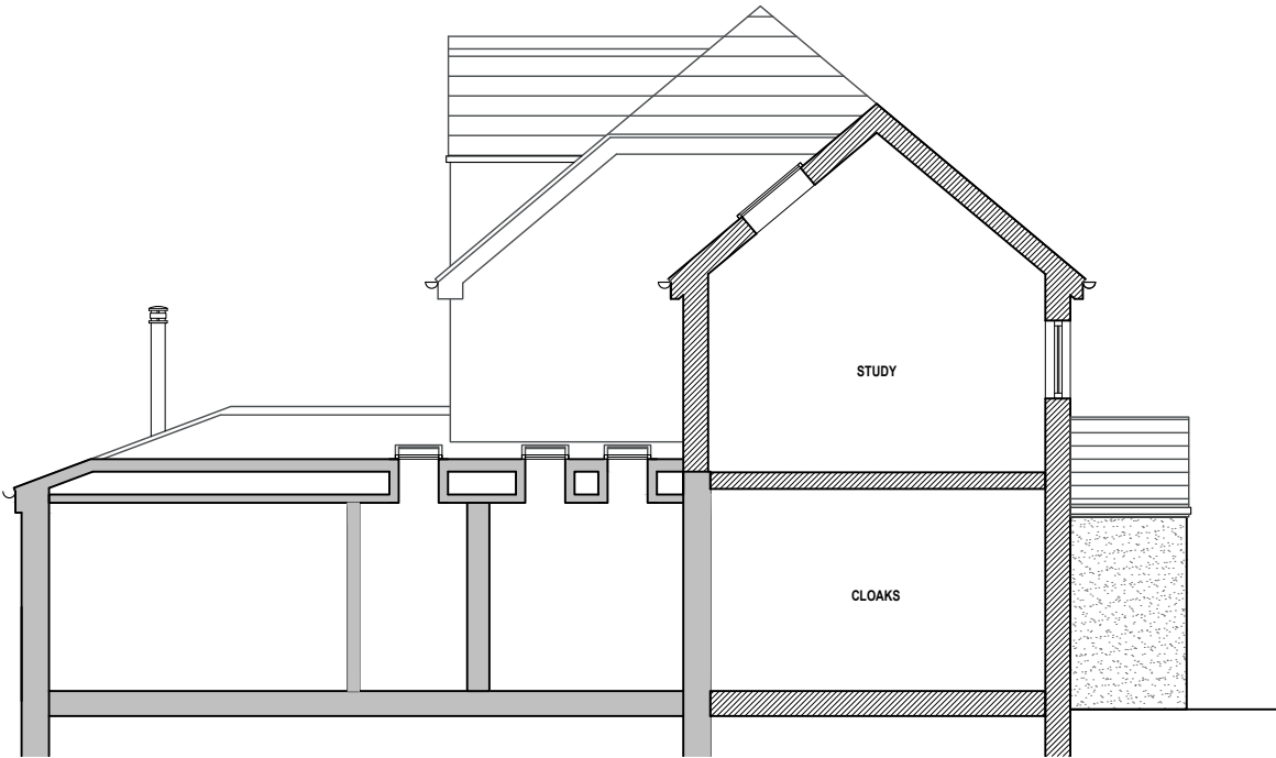
PROPOSED SECTION
