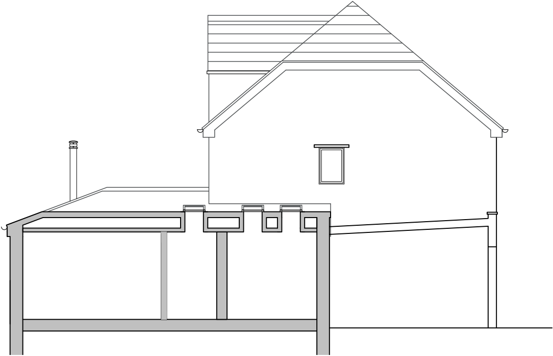
EXISTING SECTION
