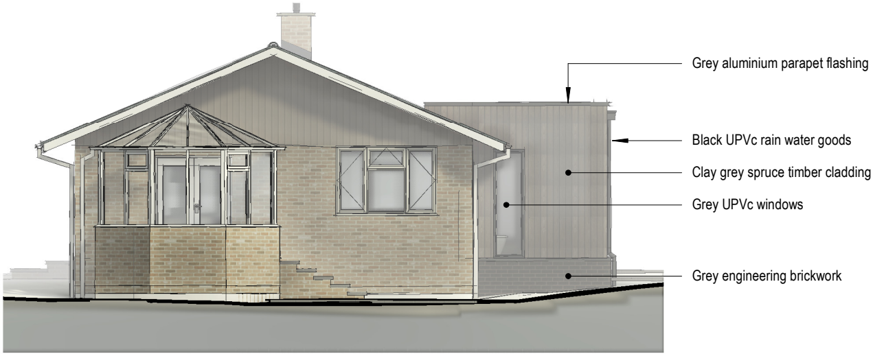
Proposed NorthEast Elevation 1 : 100
